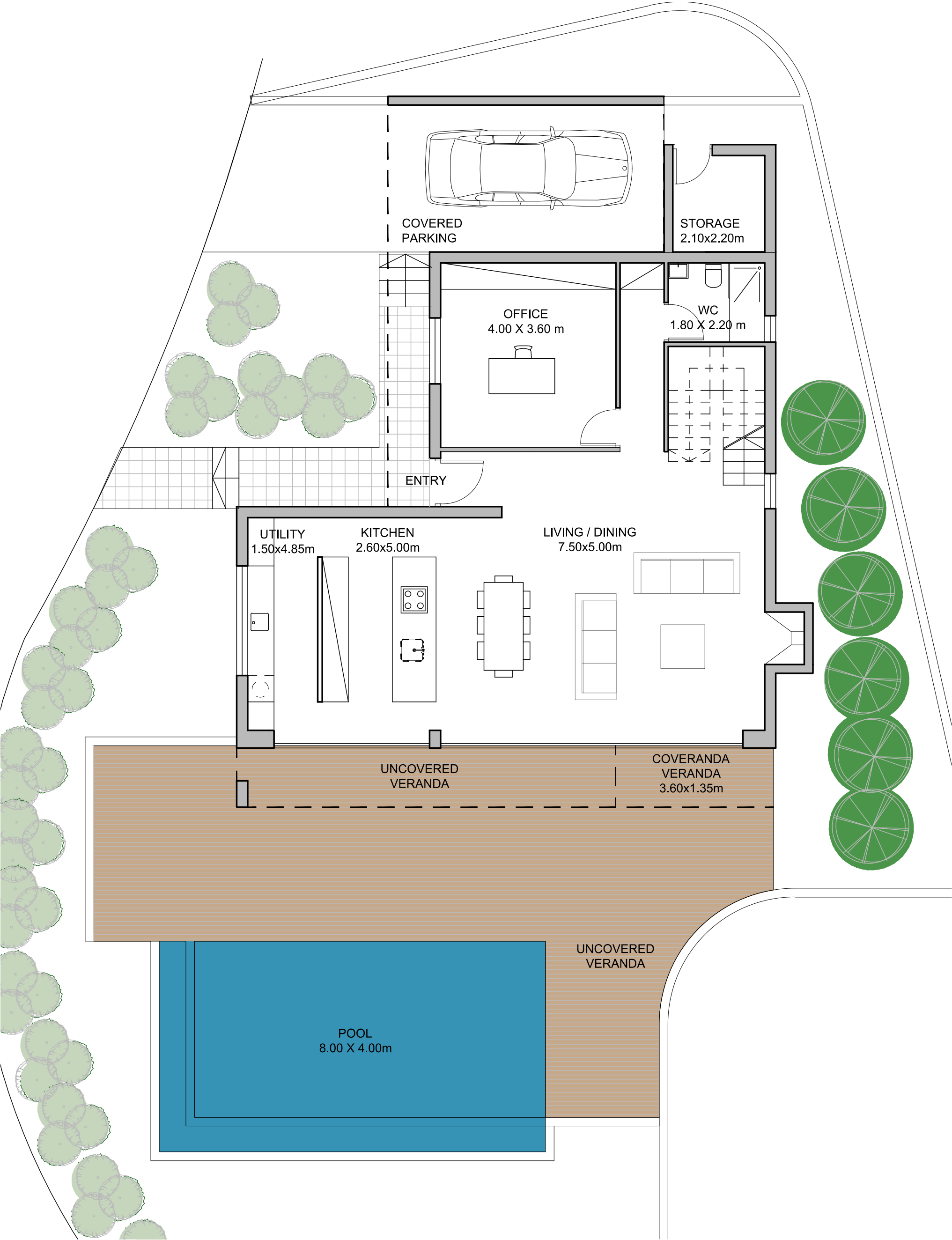
GROUND FLOOR
