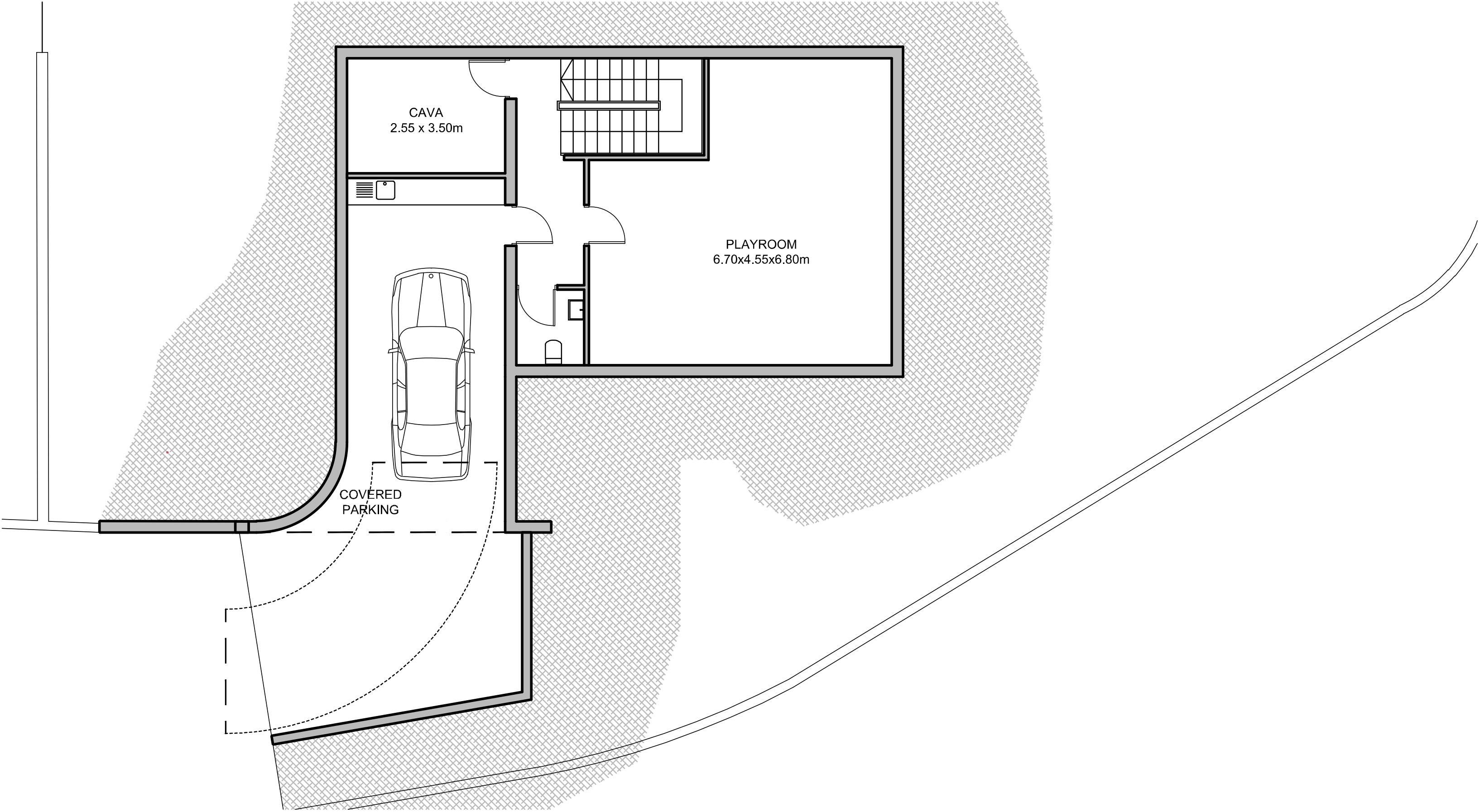
BASEMENT
